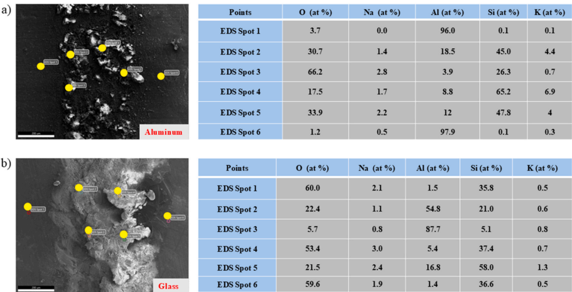
Fig. 14. EDS point analysis of the bonding interface for Sample A (Green zone).
